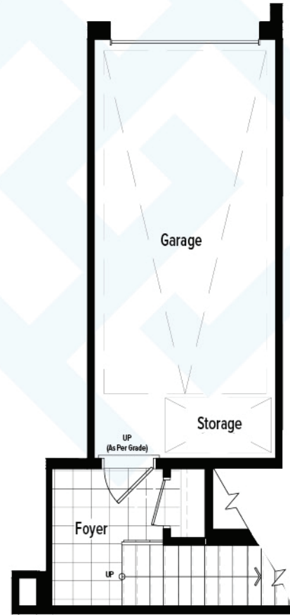
S6B - REAR ENTRY LEVEL
