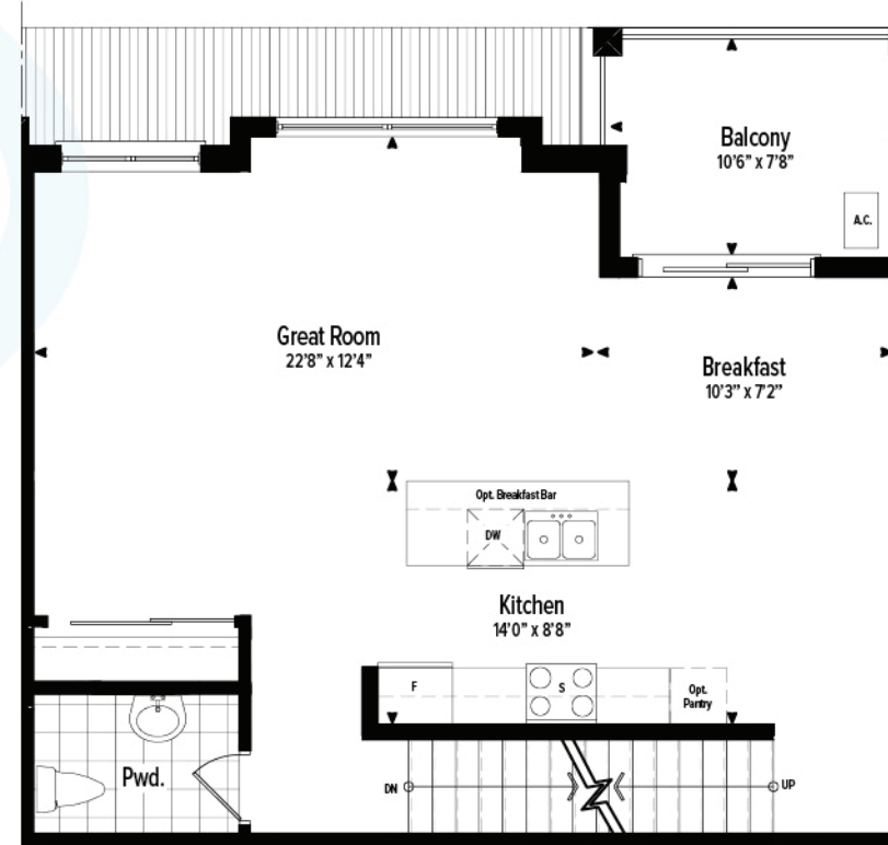
S5B - SECOND LEVEL
